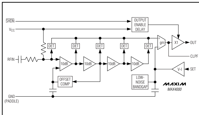
Figure 1. Functional Diagram
